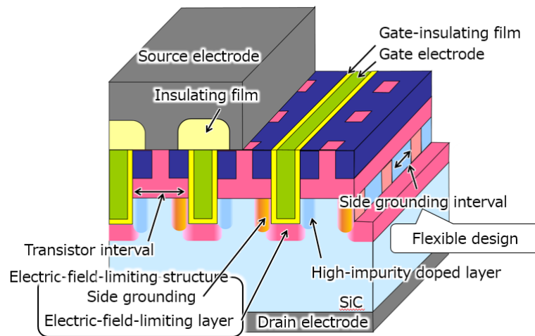
Fig. 3 Three-dimensional schematic of new trench-type SiC-MOSFET
