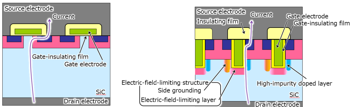
Fig. 1 Cross-sectional view of conventional planar SiC-MOSFET (left) and new trench SiC-MOSFET (right)
