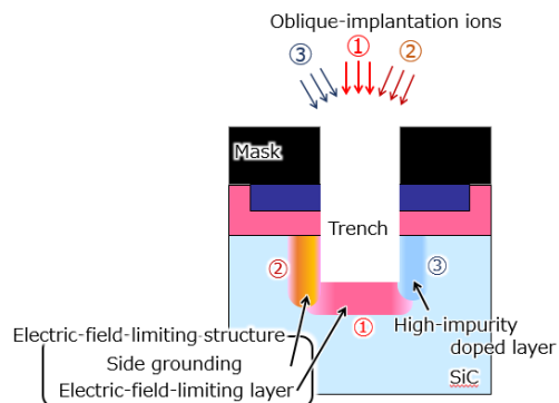
Fig. 2 Developed manufacturing method for trench type SiC-MOSFET
