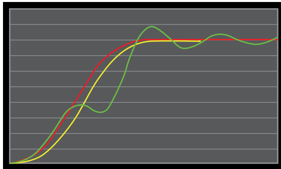
Figure 3: In the most basic form of auto-tuning, the system runs a command sequence, calculates the deviation (green) from the ideal profile (red), and develops a filter to eliminate the error and achieve proper motion (yellow).
