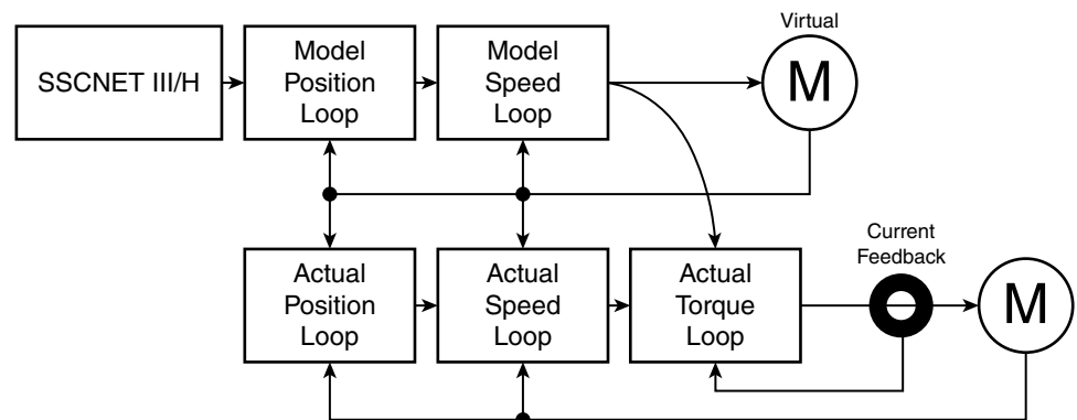
Figure 1, The MR-J4 servo drive applies the command sequence to an internal virtual servo motor (the observer) simultaneous with the real physical system, using any deviation detected in closing the speed or position loop to drive errors zero.
