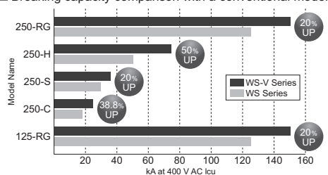
■ Breaking capacity comparison with a conventional model
